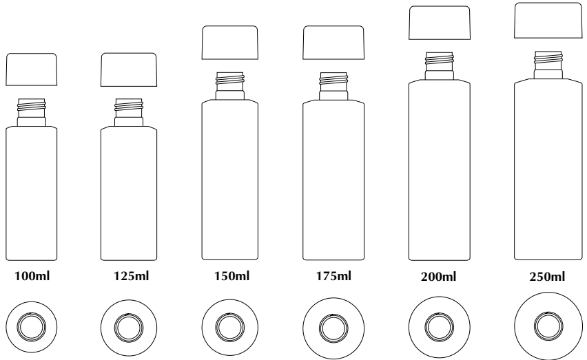
Scale 1:4 Front & Top View, & Cap
