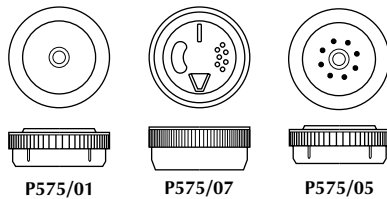
Scale 1:3 Front View & Closures
