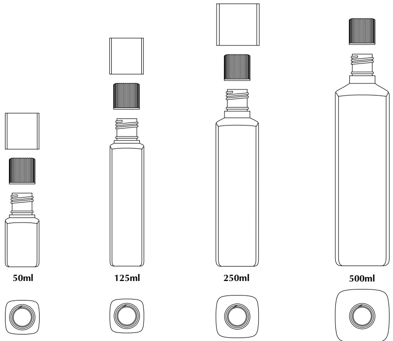
Scale 1:4 Front & Top View, Cap & Overcap
