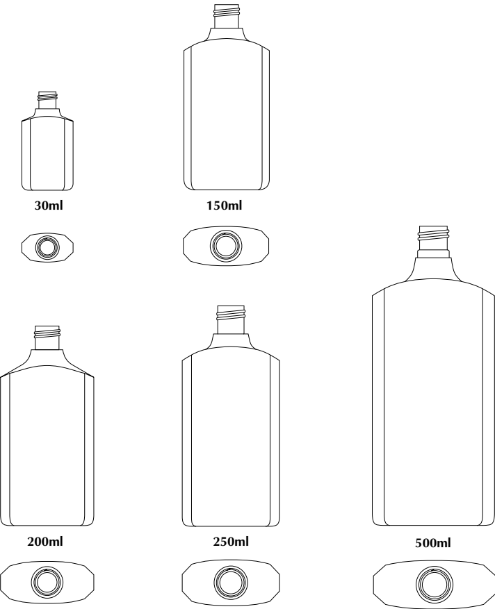
Scale 1:4 Front & Top View
